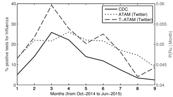
Fig. 21: T-ATAM's and ATAM's flu probability given the month and influenza rate calculated by CDC as a percentage of positive tests for flu in US
