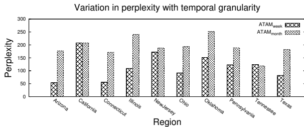
Fig. 17: Variation in perplexity for ATAM at different temporal granularities. Results for top-10 active regions.
