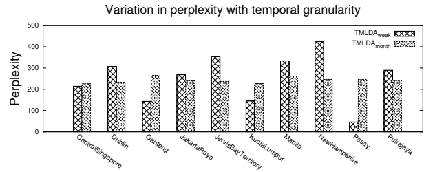
Fig. 20: Variation in perplexity achieved by TM-LDA at different temporal granularities. Results for 10 non-us active regions.
